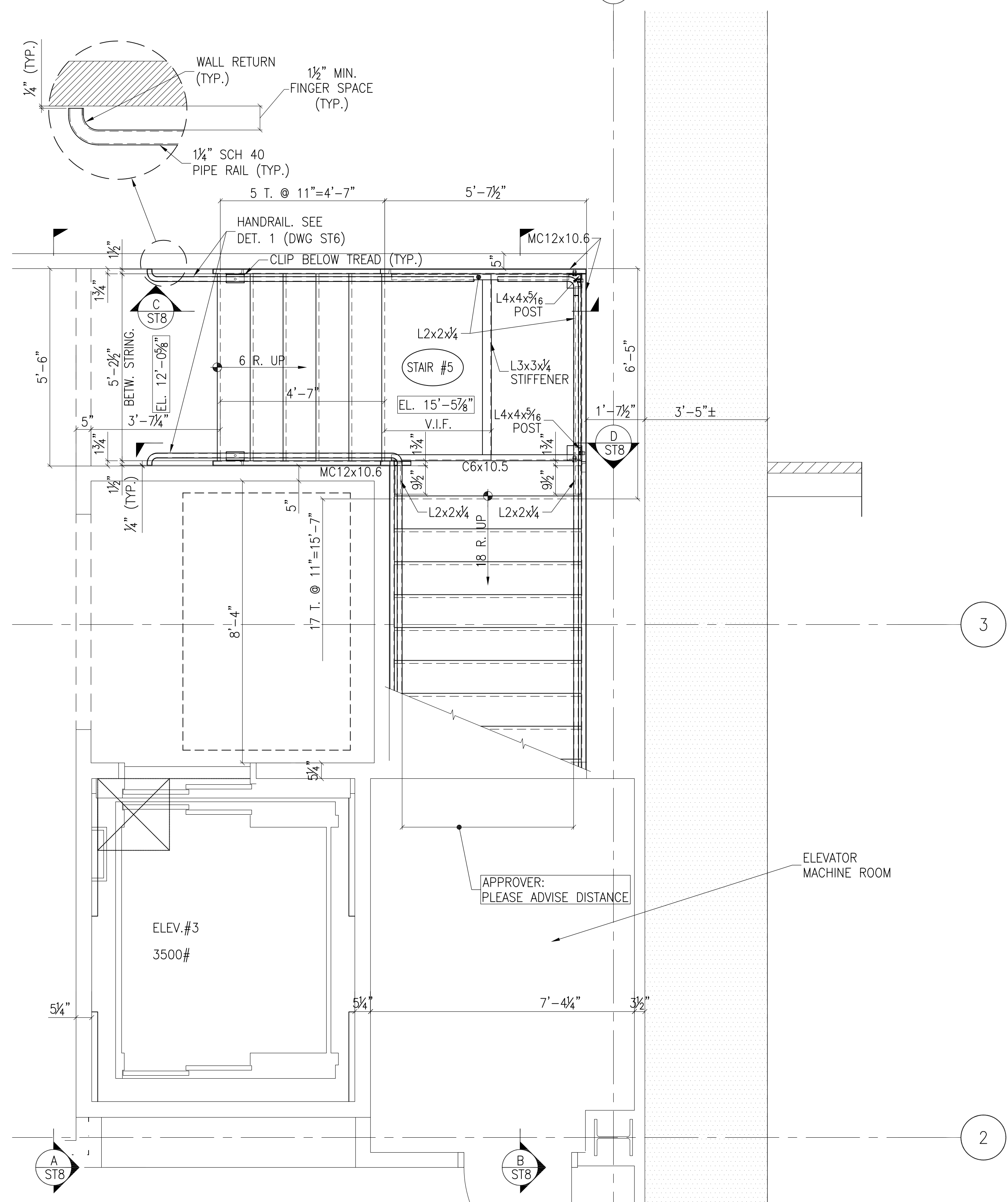
STAIR #5 PLAN AT CELLAR FLOOR SCALE: 1/2" = 1'-0"
