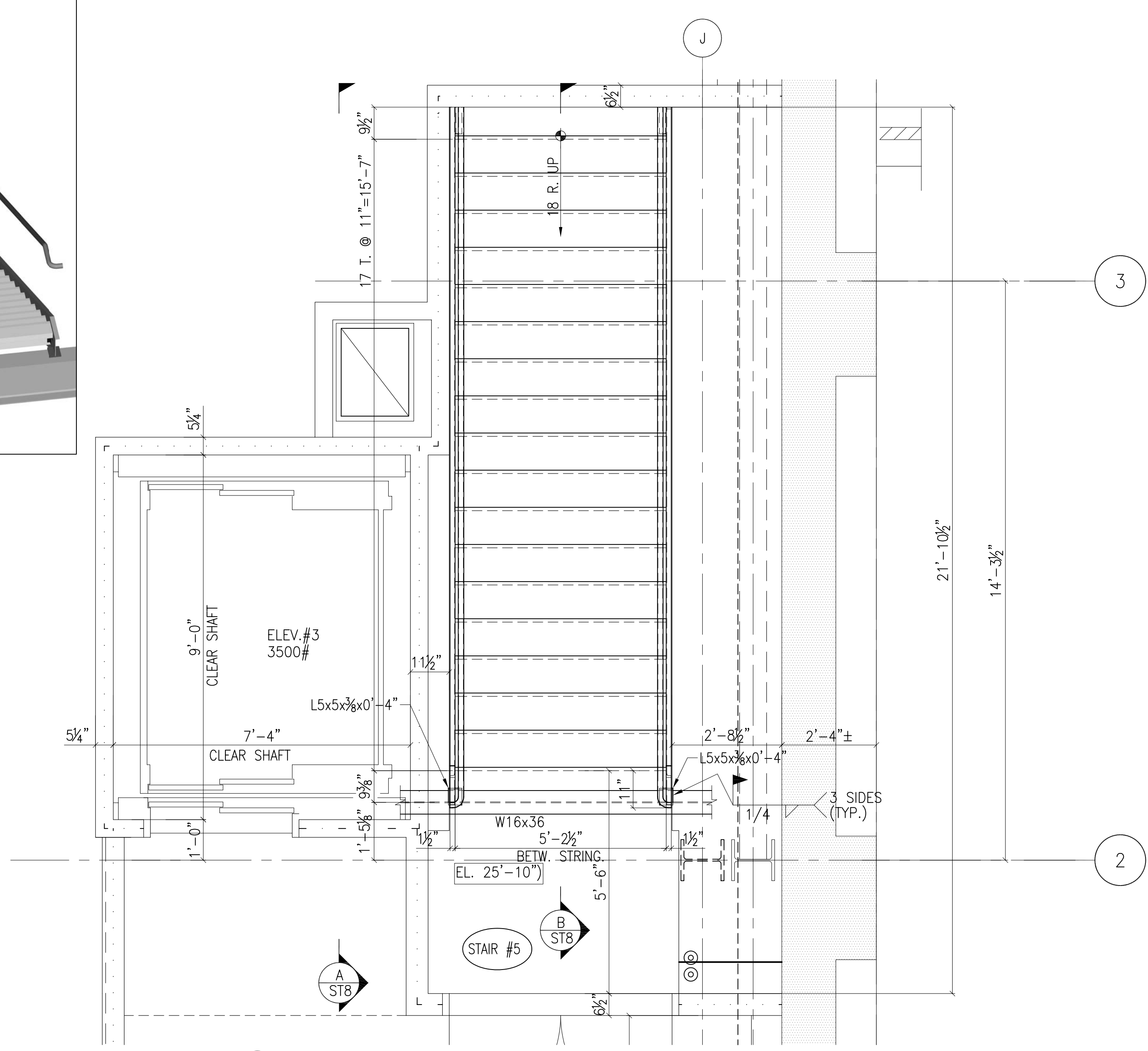
STAIR #5 PLAN AT 1ST FLOOR SCALE: 1/2" = 1'-0"
